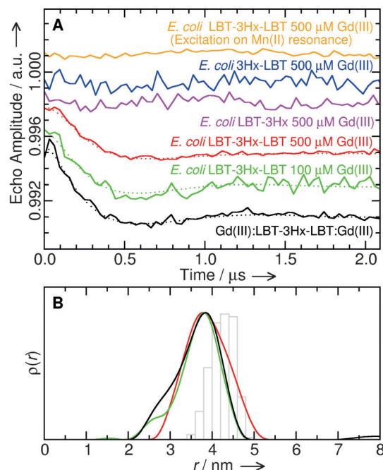
Figure 2. 94 GHz DEER measurements of E. coli cells after 4 h of induction of LBT-3Hx-LBT and 3Hx in growth medium supplemented with \text{Gd}^{\text{III}} . A) Background-corrected DEER time traces (solid line) and fits (dashed lines) based on the \text{Gd}^{\text{III}} - \text{Gd}^{\text{III}} distance distributions from Tikhonov analysis shown in (B), together with the distance probability histograms (gray) obtained from molecular dynamics. The time trace of purified 200 \mu\text{M} \text{Gd}^{\text{III}} :LBT-3Hx-LBT- \text{Gd}^{\text{III}} is shown in black.
