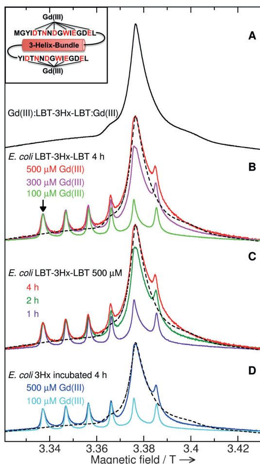
Figure 1. 94 GHz 4.5 K field-swept echo-detected EPR spectra of \text{Gd}^{\text{III}} :LBT-3Hx-LBT- \text{Gd}^{\text{III}} A) purified (black and black-dashed in other panels); B) in E. coli cells after 4 h induction on medium supplemented with the indicated \text{Gd}^{\text{III}} concentrations; and C) after various induction times on media supplemented with 500 \mu\text{M} \text{Gd}^{\text{III}} . D) The spectrum for 3Hx in E. coli cells after 4 h induction on medium supplemented with the indicated \text{Gd}^{\text{III}} concentrations is shown for comparison. All cell spectra were normalized to the intensity of the \text{Mn}^{\text{II}} resonances. The inset shows the LBT sequences with the \text{Gd}^{\text{III}} -coordinating residues in red.
